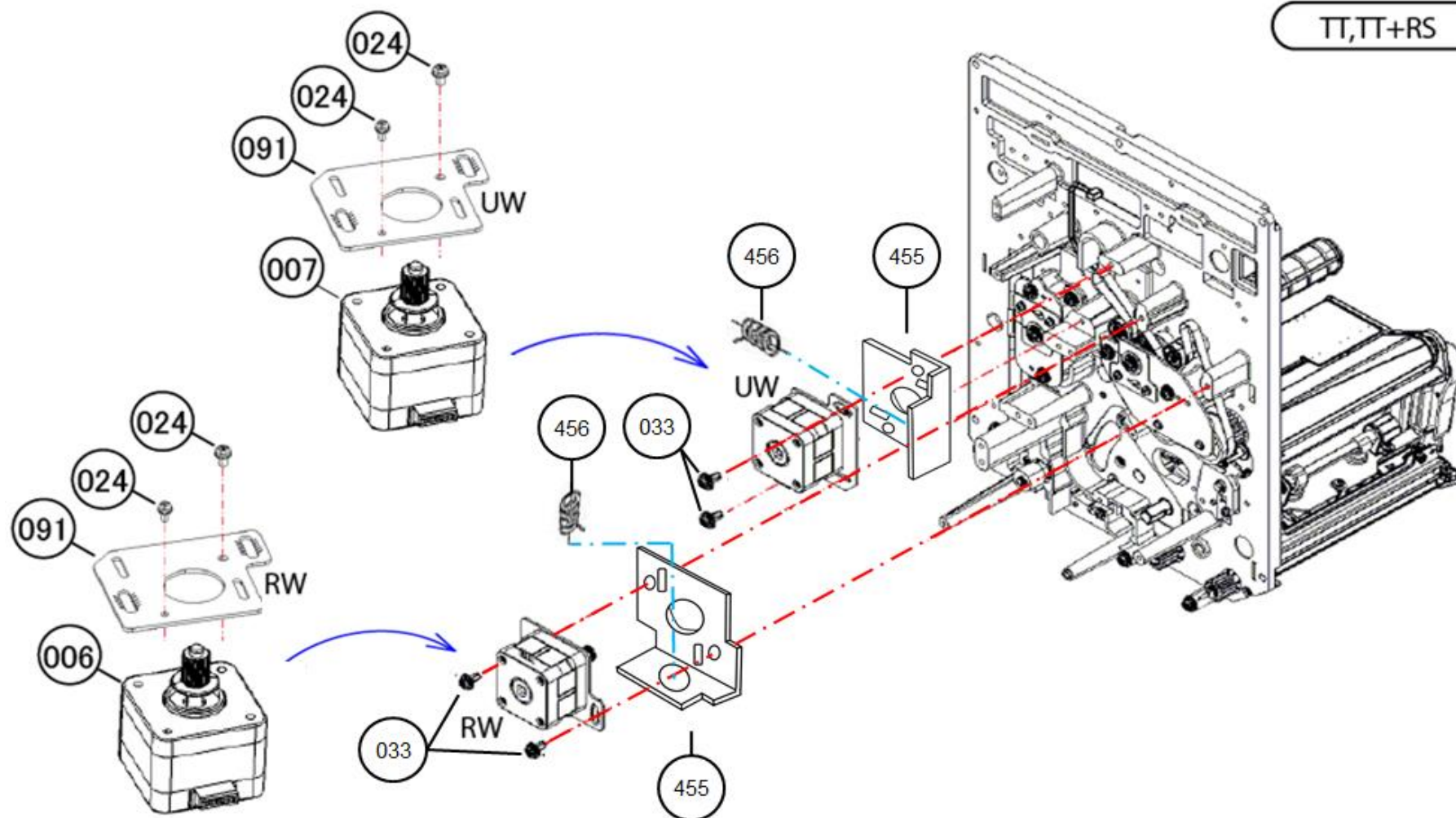
DESCRIPTION Fig42-RH Ribbon③
