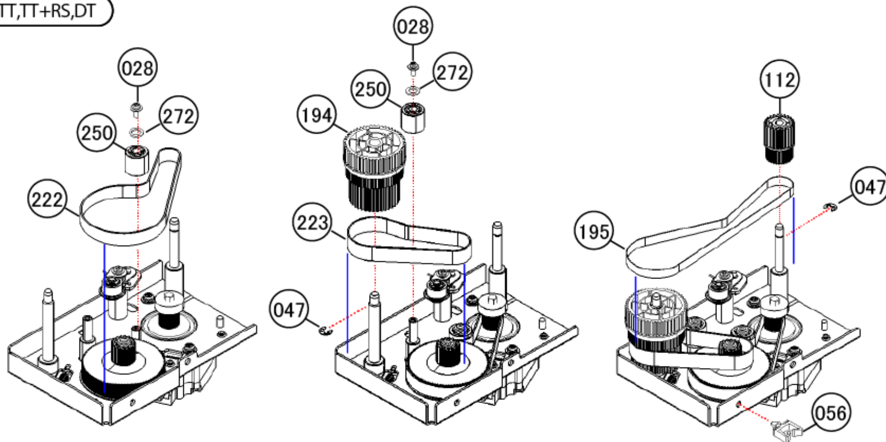
DESCRIPTION Fig47-LH Gear Box②
