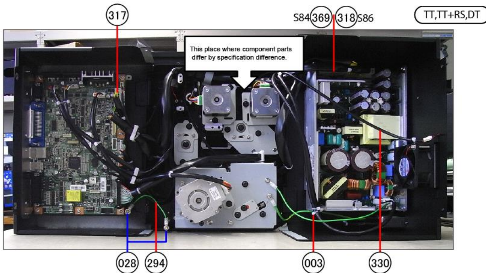
DESCRIPTION Fig68-RH Cable②
