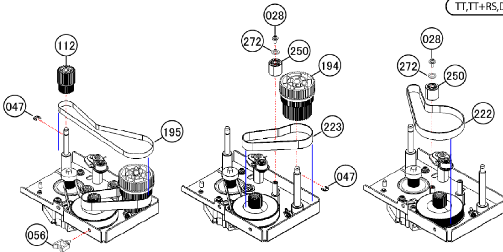
DESCRIPTION Fig48-RH Gear Box(2)
