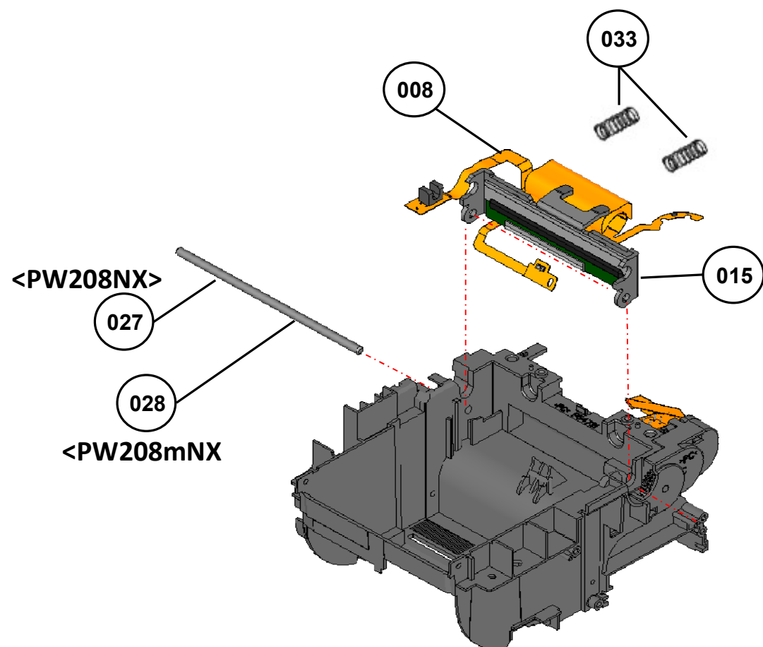
DESCRIPTION Fig02-ASSY
